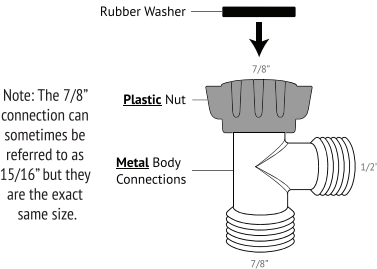
Hybrid Cold Water T-adapter (7/8" x 7/8" x 1/2")
